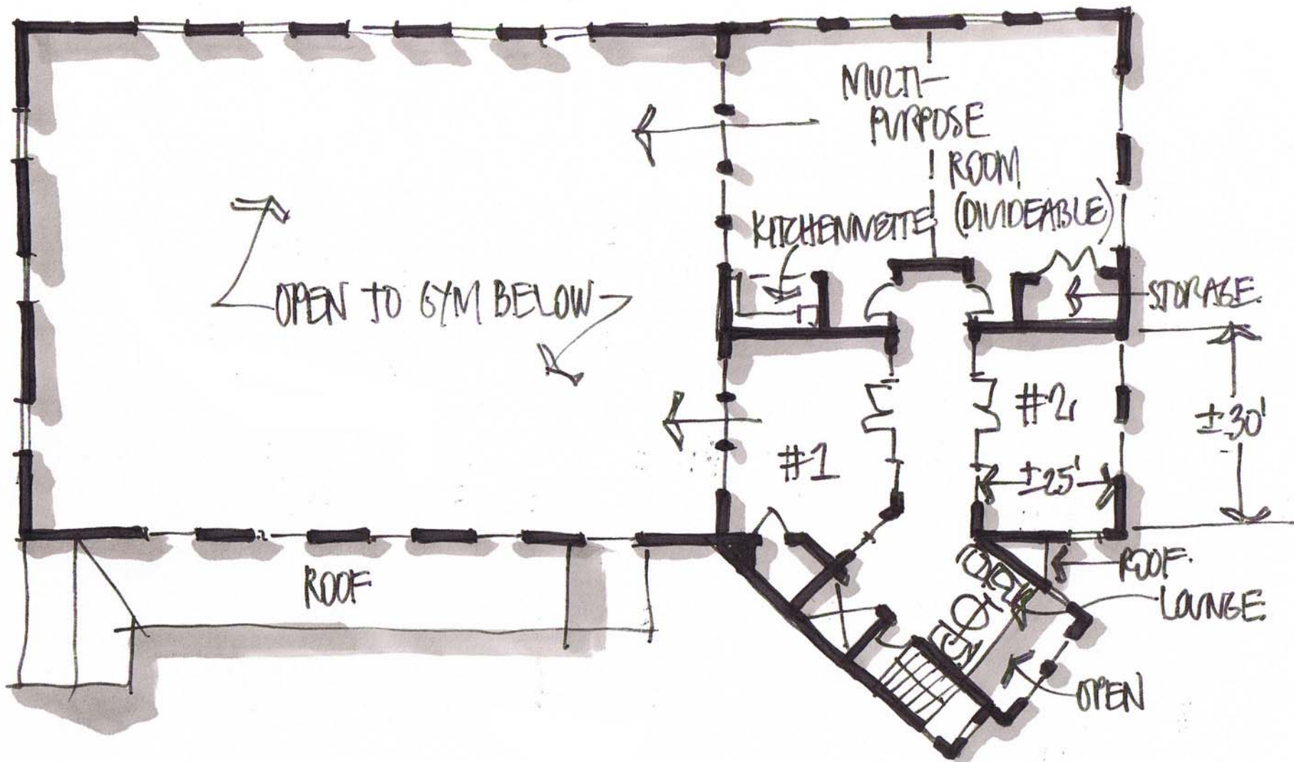
LEVEL TWO FLOOR PLAN. 5.1.07 1" = 20'
